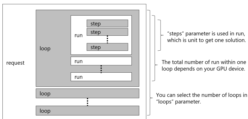
Figure 4. Computation structure of the SQBM+ computation API
