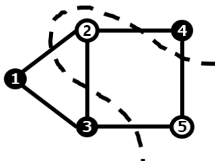
Figure 5. MAX-CUT problem
