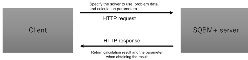
Figure 2. Example of using the SQBM+ computation API
